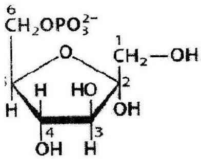
Fructose 6-phosphate
