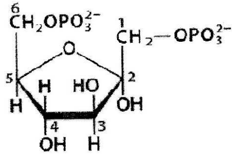
Fructose 1,6-bisphosphate
