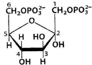
Fructose 1,6-bisphosphate
